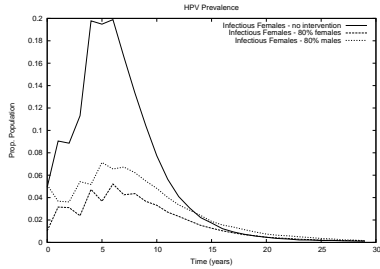
Figure 2. Population-level impact of HPV interventions
